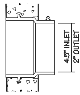
RUBBER BOOT DETAIL
