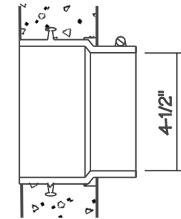
RUBBER BOOT DETAIL
