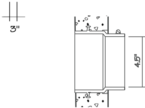
RUBBER BOOT DETAIL
